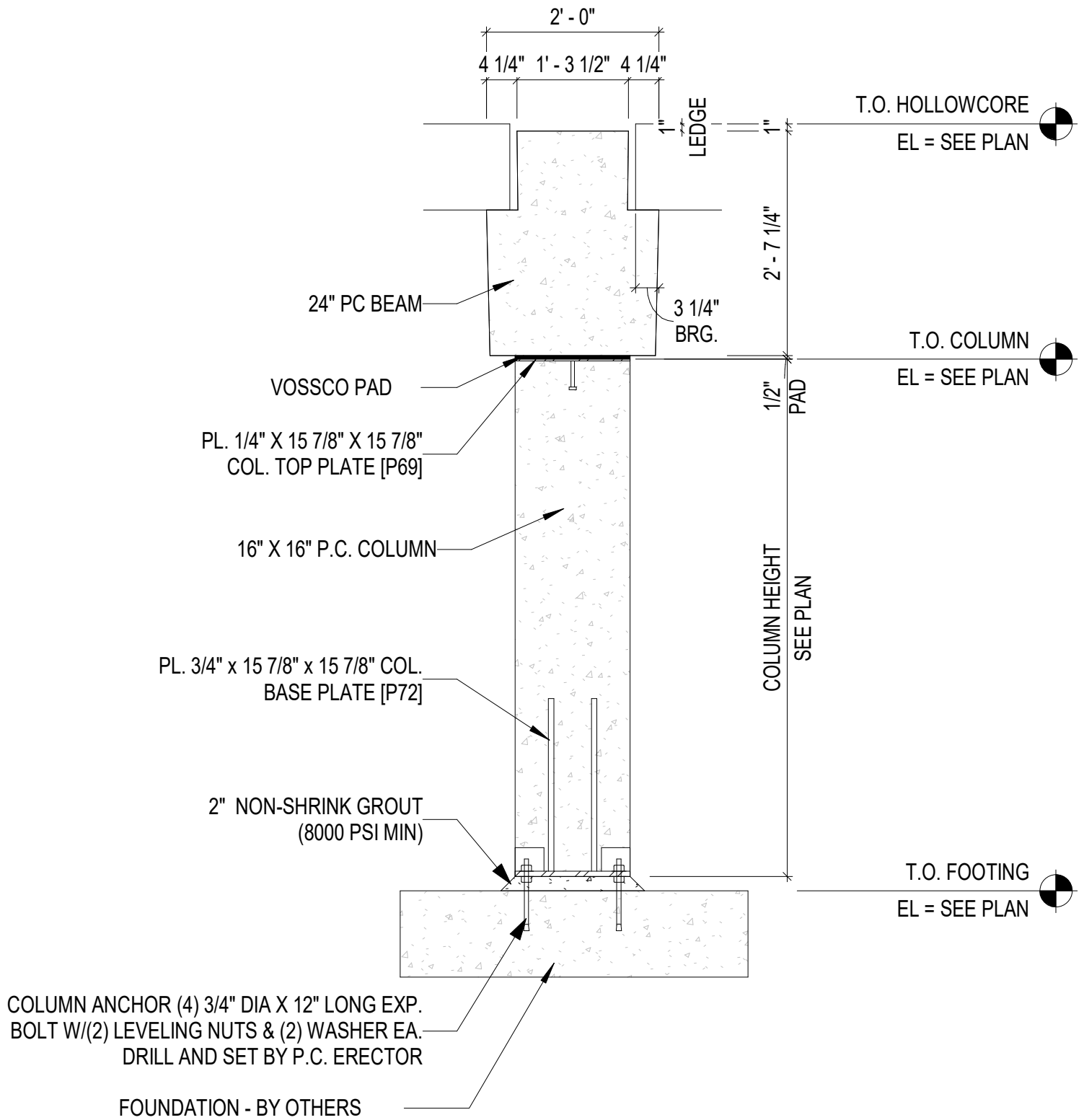
1 BEAM & COLUMN DETAIL
