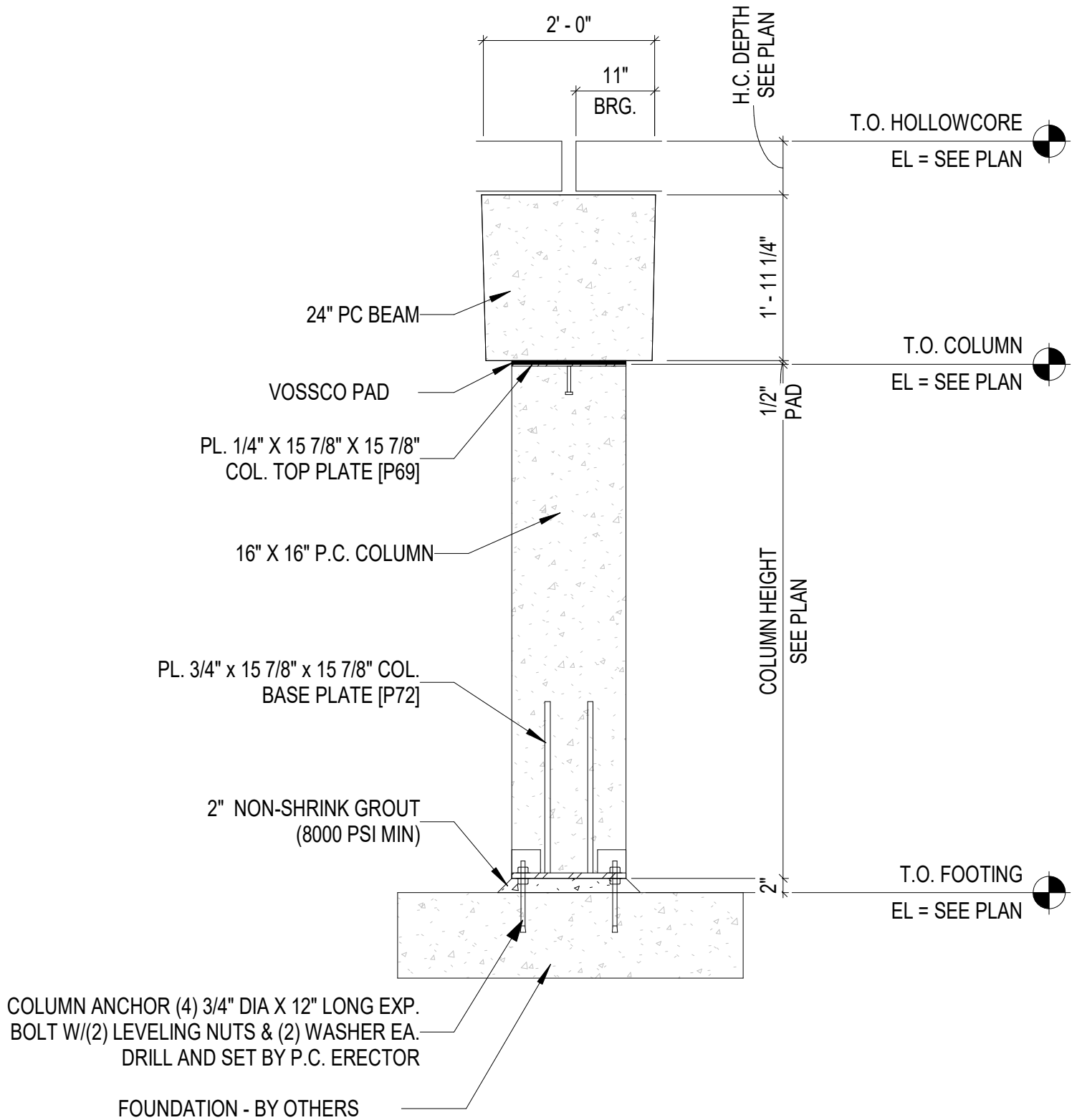
3 BEAM & COLUMN DETAIL
