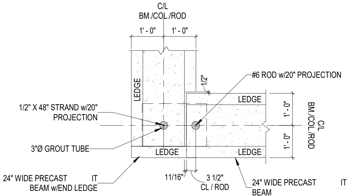
8 BEAM & COLUMN DETAIL
