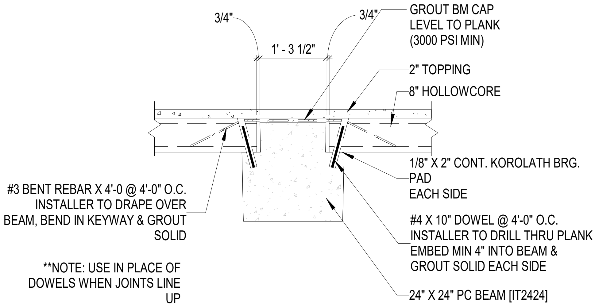
2 PLANK BRG & LAP ON PC BEAM
