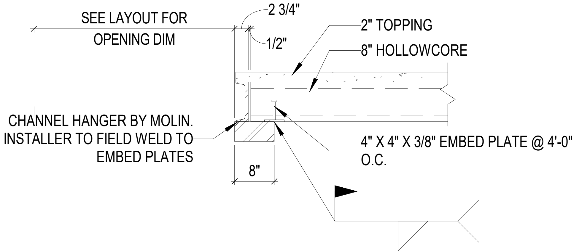
1 PLANK HANGAR CONNECTIONS
