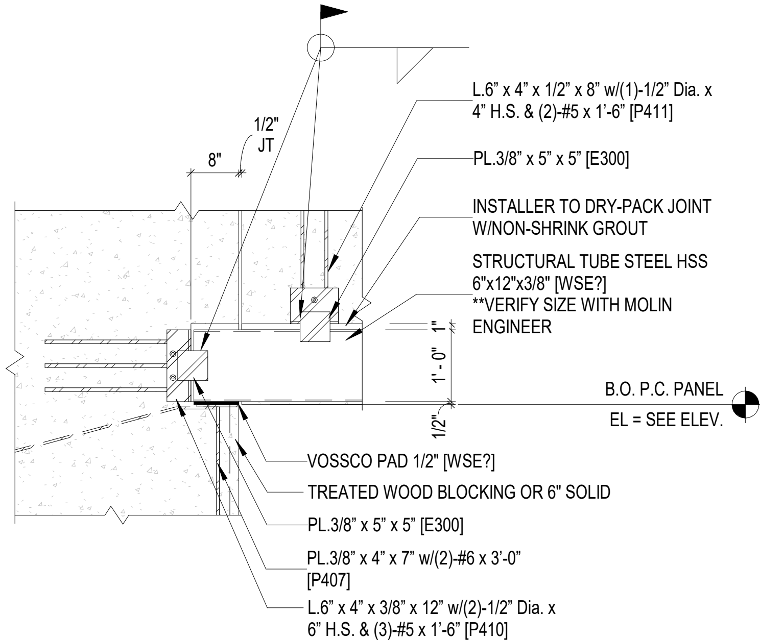
1 STEEL HEADER CONNECTION 1
