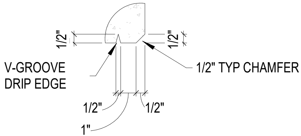
TYP. @ HEAD CONDITION
