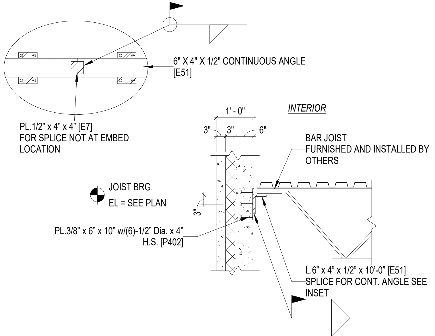
1 JOIST/GIRDER CONNECTION
